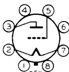
BOTTOM VIEW (G-5S 8 )
